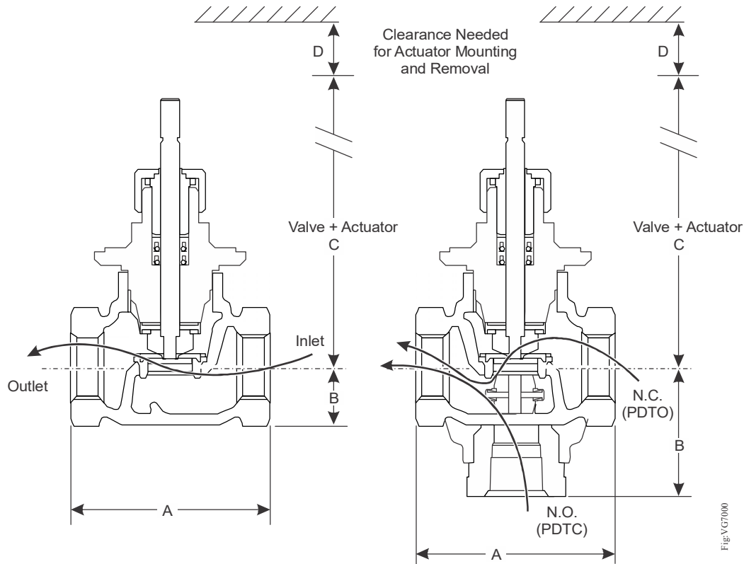
Figure 2: Two-Way Normally Open (N.O.)/Push-Down-to-Close (PDT), Two-Way Normally Closed (N.C.)/Push-Down-to-Open (PDTO), and Three-Way Mixing Valve Dimensions, Fluid Flow Directions, and Port Designations (See Table 1 and Table 2.)
